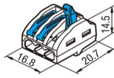
3-PORT (L13)
