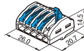
5-PORT (L15)
